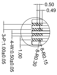
Detail A SCALE 3:1
